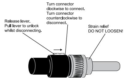
Fig 7. Speaker/LED connector
