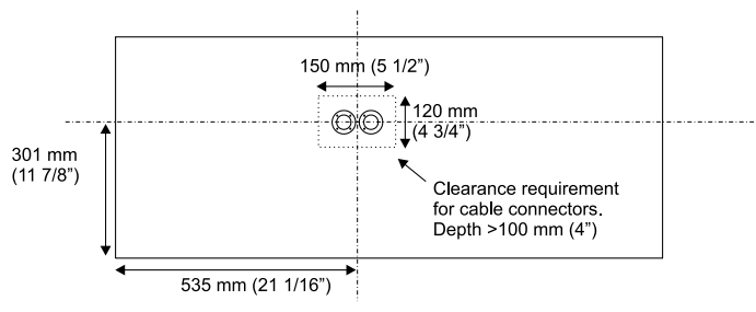
Fig 6. Recess for loudspeaker connectors. (Rear view)
