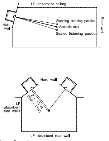
Fig 3. Speaker mounting.
