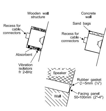
Fig 4. Speaker mounting details.
