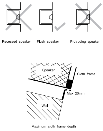
Fig 5. Eliminating discontinuities.
